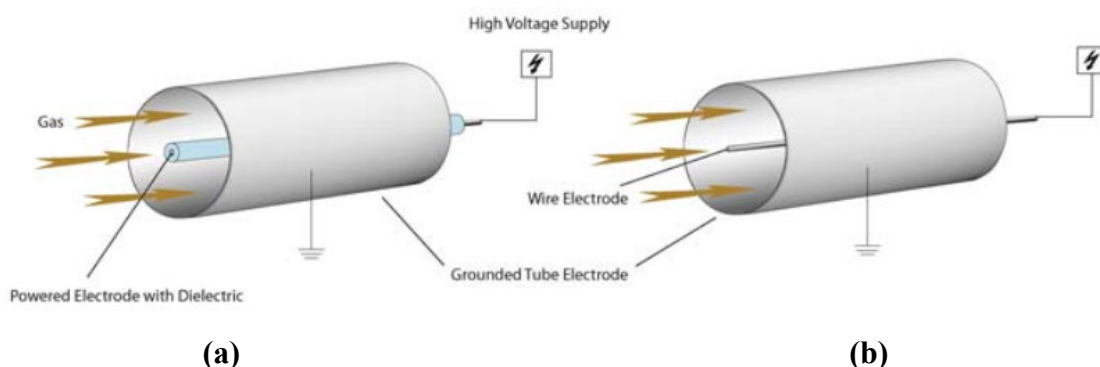
Figure 5. (a) dielectric barrier discharge (DBD) (b) corona discharge plasma
