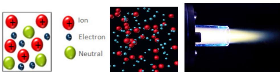
Figure 3. (a) mixture of ions, electrons and neutral atoms (b) plasma form
