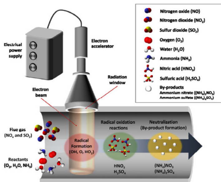
Figure 4. Flue gas removal by electron beam
