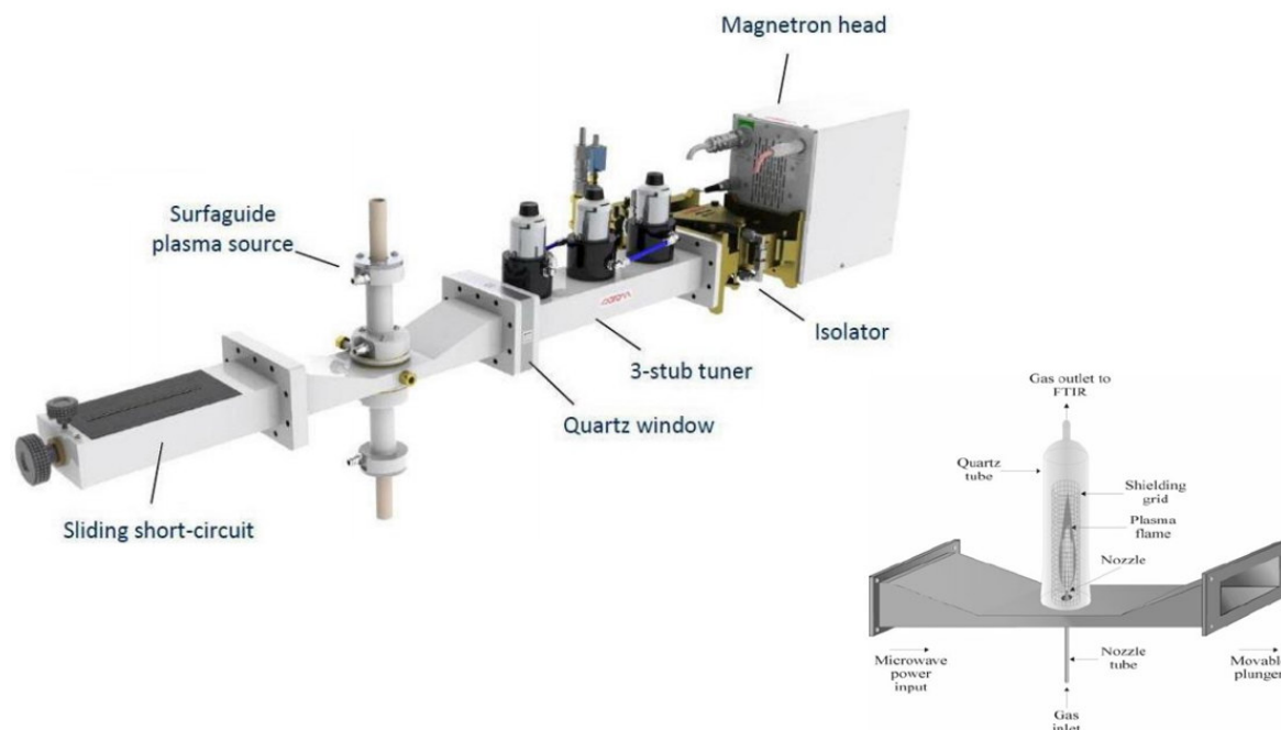
Figure 6. Microwave plasma system
