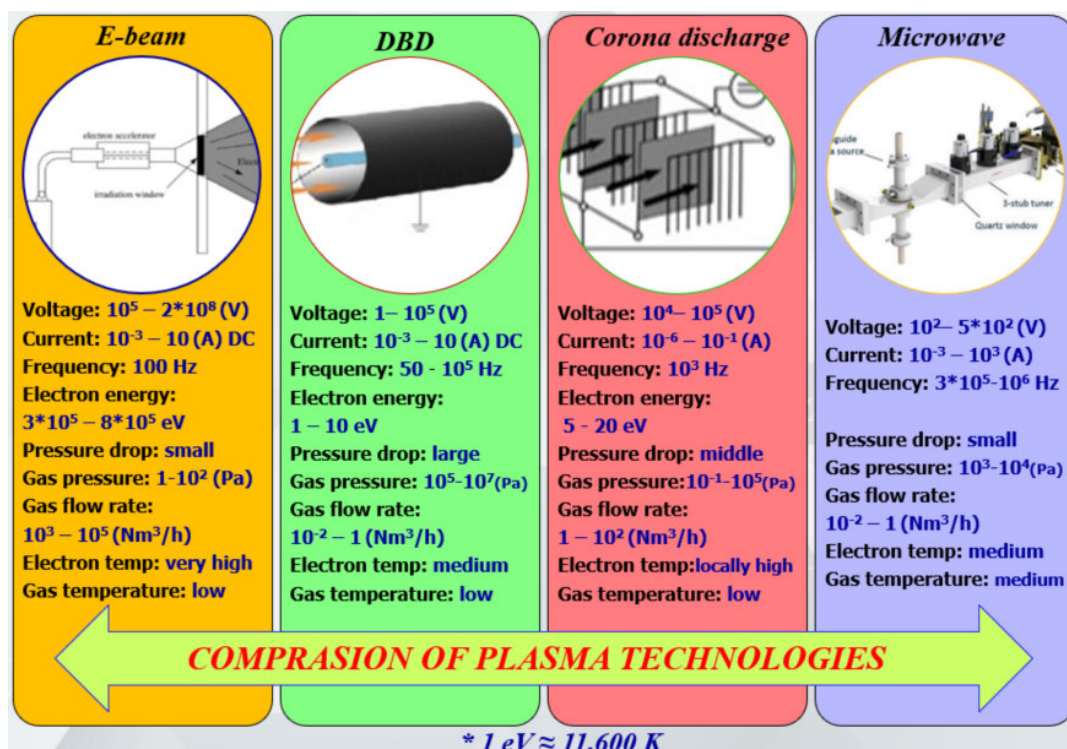
Figure 7. Comprasion of electron beam, DBD, corona discharge and microwave plasma
