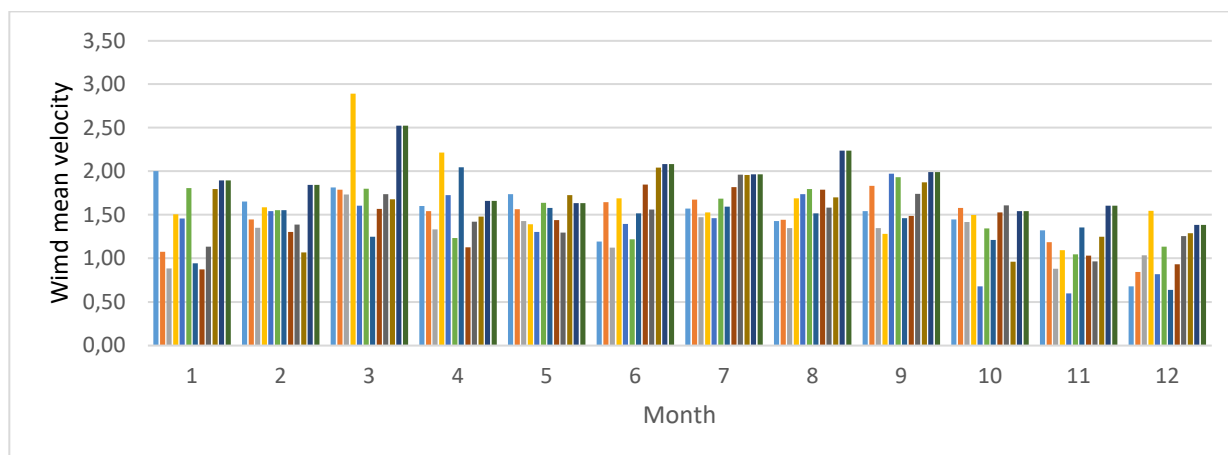
Fig.4. Wind mean velocity distribution in Gori (1993-2017)
