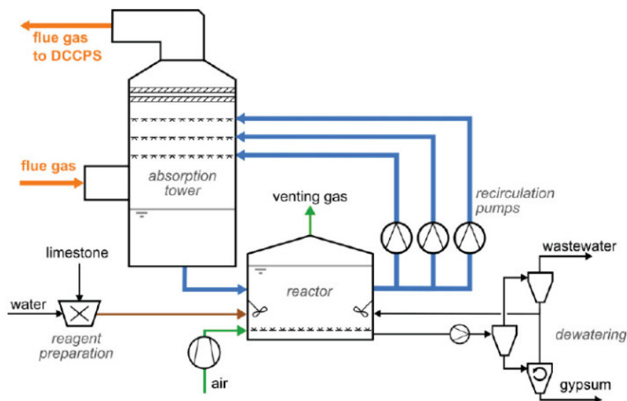
Figure 2. Flue gas desulphurization (FGD) system
