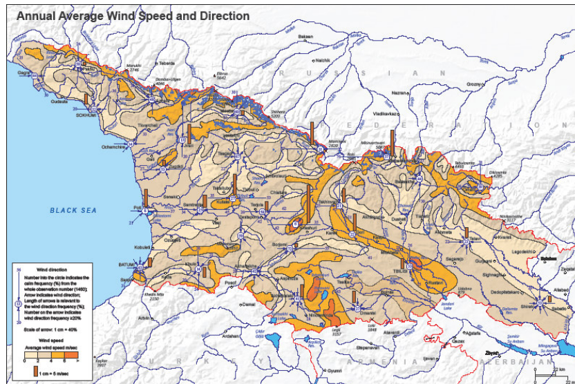
Fig.2. Wind velocity and direction GIS map
