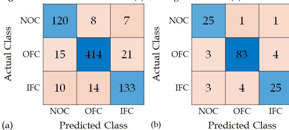
Figure 2. Confusion matrices for (a) training dataset and (b) test dataset.
